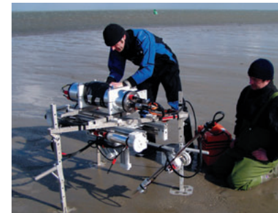
The instrument "Lance-A-Lot" maps structures at the sediment surface (e.g., ripples, mounds or pits) using a laser beam and a digital camera.
