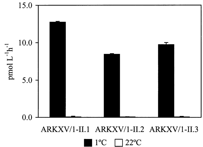
Fig. 3. Bacterial ^3\text{H} -leucine uptake in melt pools ARKXV/1.11.1–11.3 that were incubated for 12 h at 1°C and 22°C.
